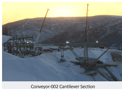
Conveyor-002 Cantilever Section
